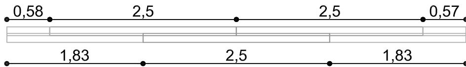
Trame bardage x 14
